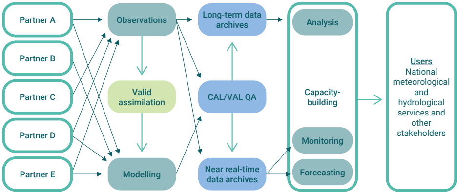
Figure 32. WMO SDS-WAS regional node operation concept
