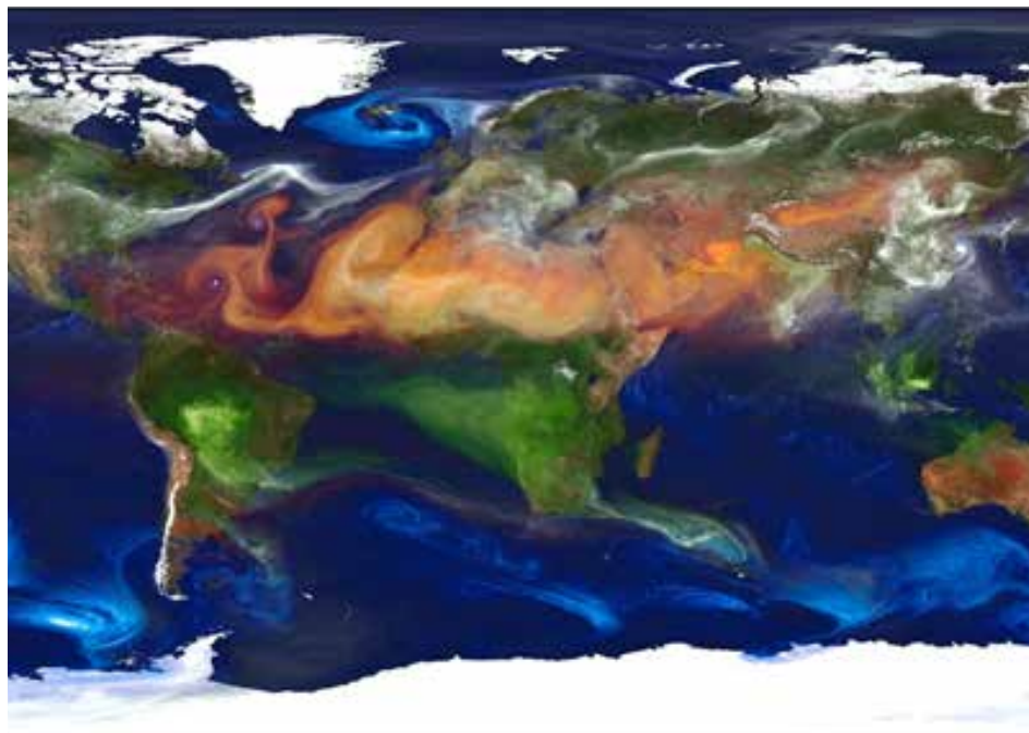
Figure 2. Aerosol optical thickness
