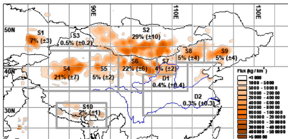
Figure 4. Sources (S1 to S10) and typical depositional areas (D1 and D2) for Asian dust aerosol associated with spring average dust emission flux ( \text{kg km}^{-2} \text{ spring}^{-1} ) between 1960 and 2002
