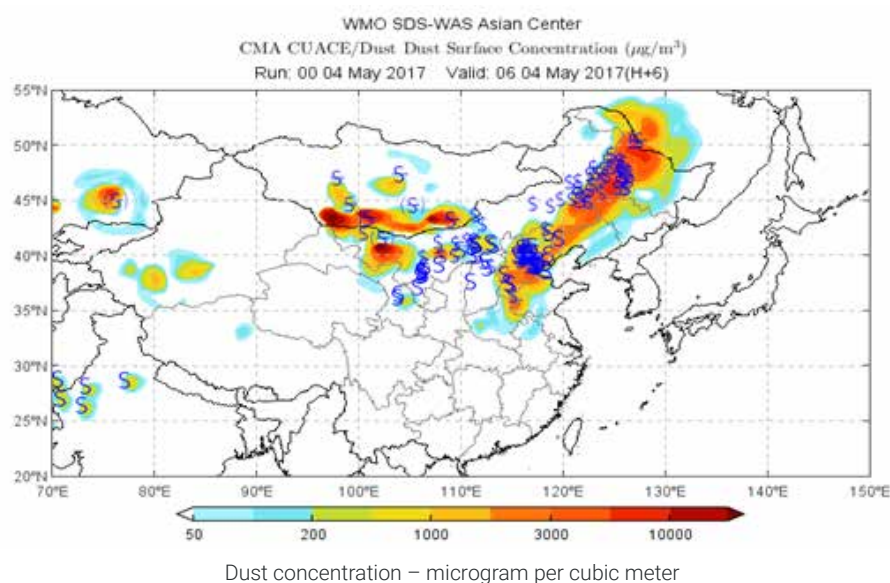
Figure 37. Verification of a dust forecast released by the CUACE 34 / dust model with surface SDS observational data from meteorological stations
